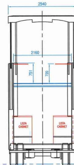
SECTIONAL END ELEVATION WITH ROOF RAISED
