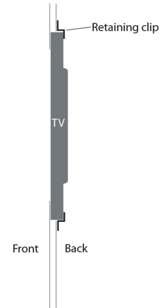
Cross section, Double sided panel with TV
